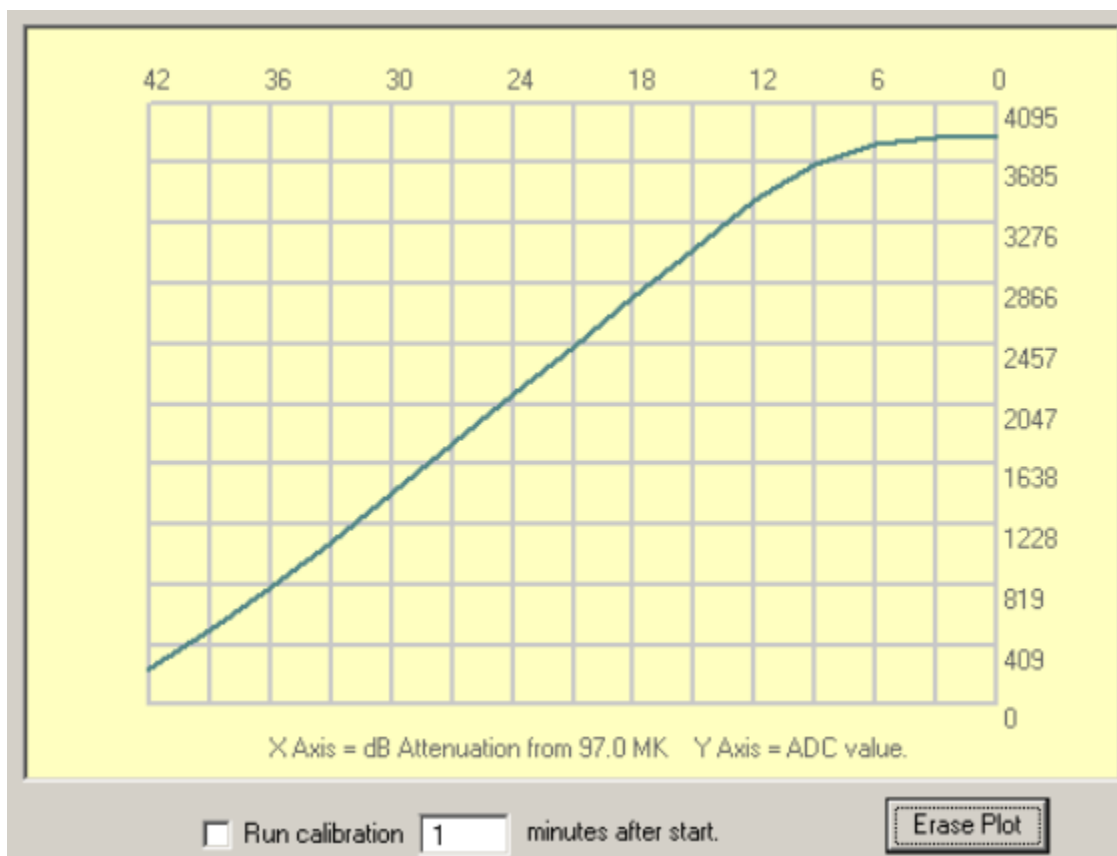
Illustration 28: Plot window from the Calibrator Control panel. In this plot we can see that gain compression is occurring at the higher noise levels.
