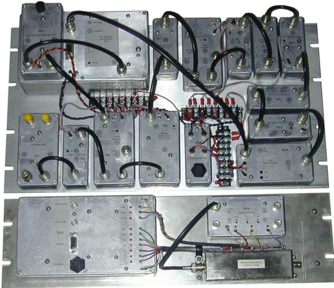
Illustration 42: FS200B production model spectrograph with an automated step calibrator on the bottom panel. Everything can be controlled remotely via the serial port attached PC. From the front of the rack you just see an led, reset button, and perhaps a switch (can't remember). Basically, a DDS controls a receiver with a log detector. A micro-controller manages everything.
