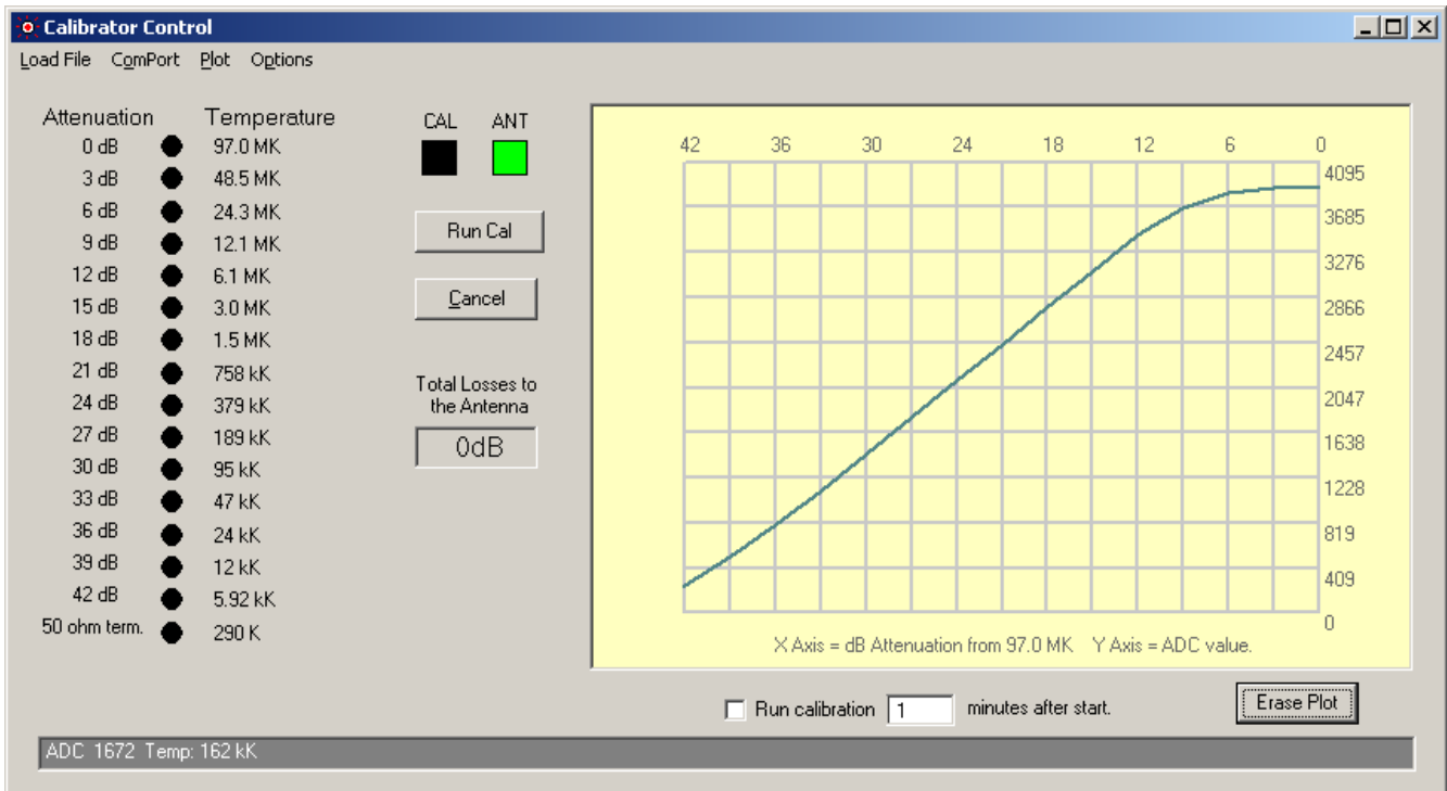
Illustration 23: The Calibrator Control panel allows automatic calibration of Radio-Sky Spectrograph when connected to the MK2 calibrator.
