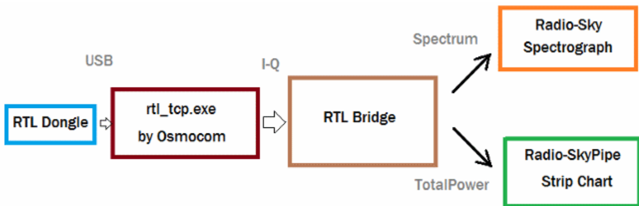
Illustration 36: Diagram of data flow when using RTL Bridge.
