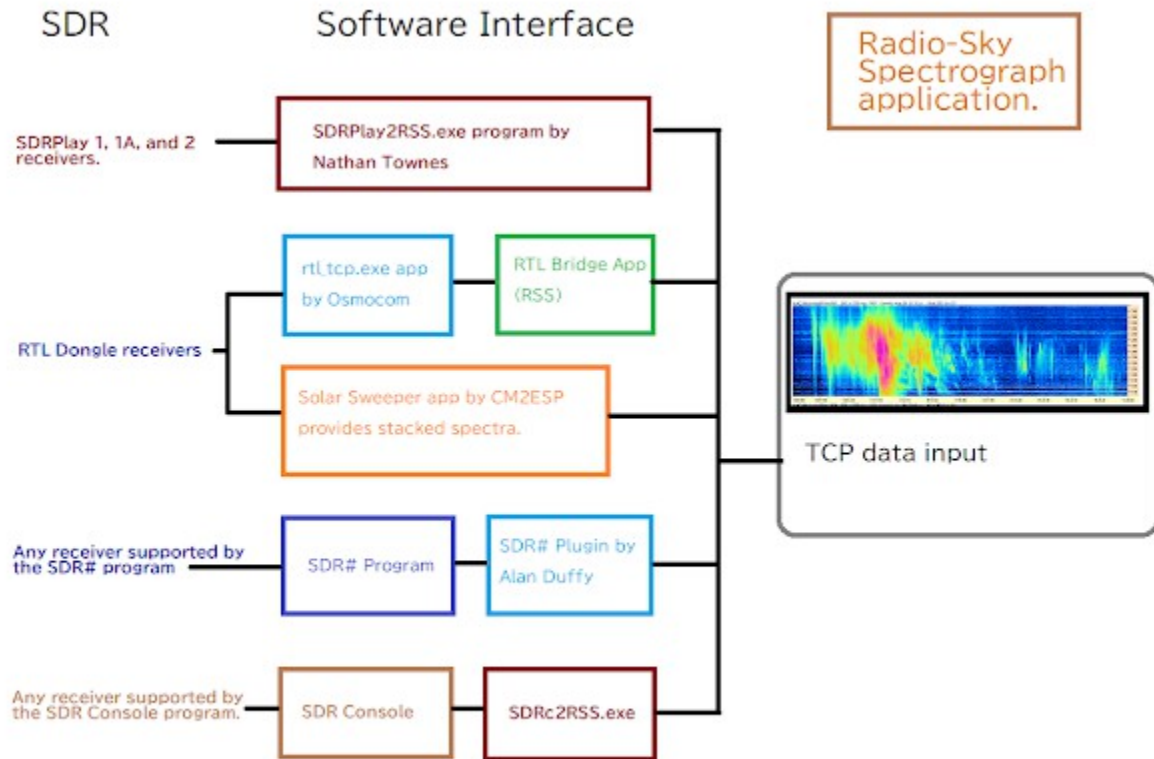
Illustration 17: Diagram of SDR to Radio-Sky Spectrograph interfaces.
