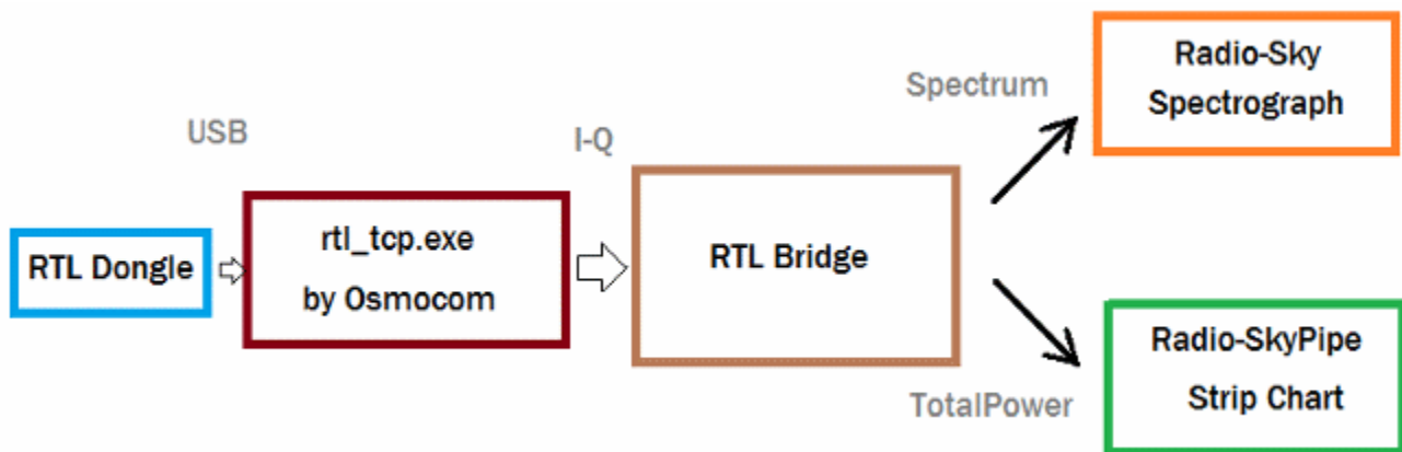
Illustration 35: Diagram of data flow when using RTL Bridge.
