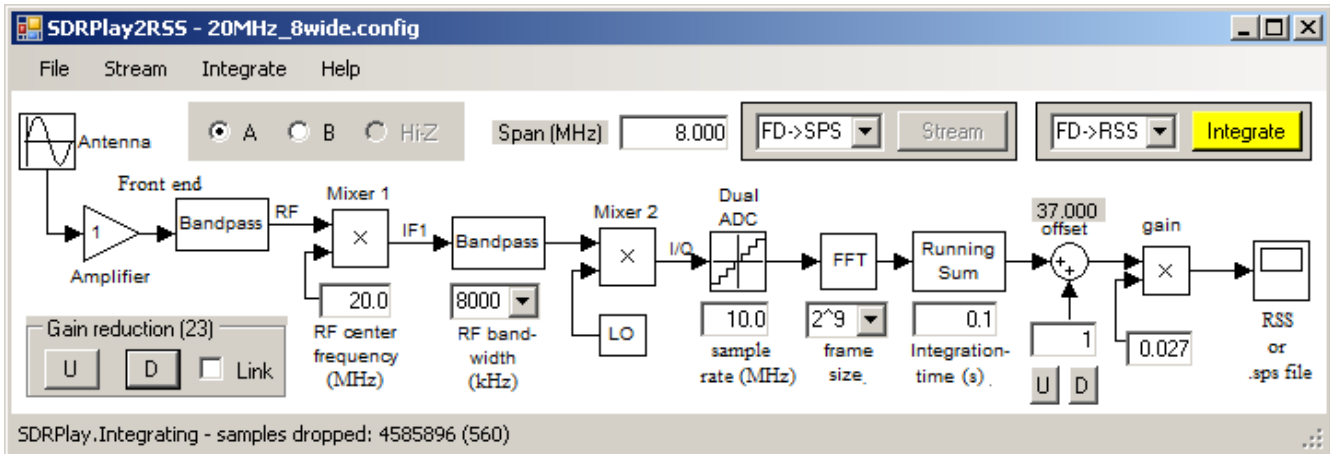
Illustration 39: SDRPlay2RSS application. The yellow Integrate button indicates the active connection with the SDRPlay receiver.
