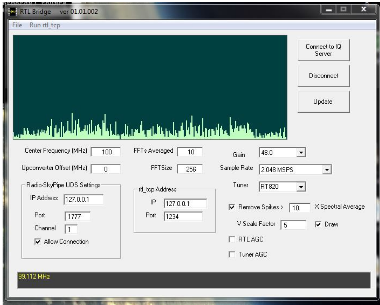
Illustration 36: RTL Bridge window.
