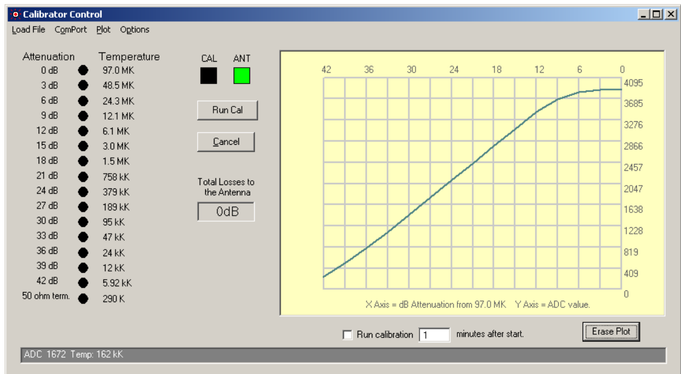
Illustration 22: The Calibrator Control panel allows automatic calibration of Radio-Sky Spectrograph when connected to the MK2 calibrator.
