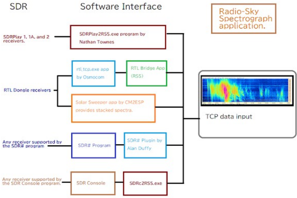
Illustration 16: Diagram of SDR to Radio-Sky Spectrograph interfaces.
