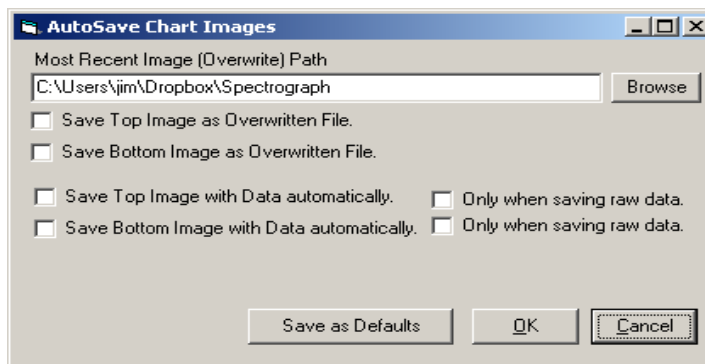
Illustration 21: The AutoSave Chart Images window controls where and how spectrogram image files are automatically saved.
