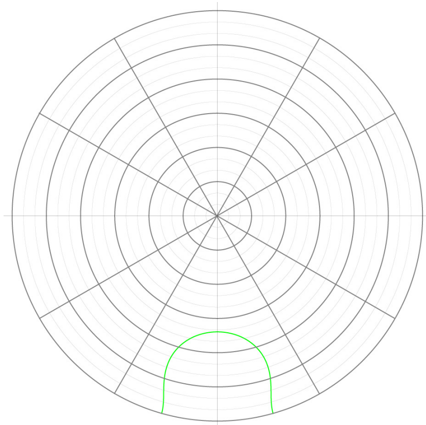
TFD Array Beam Shape 65S
