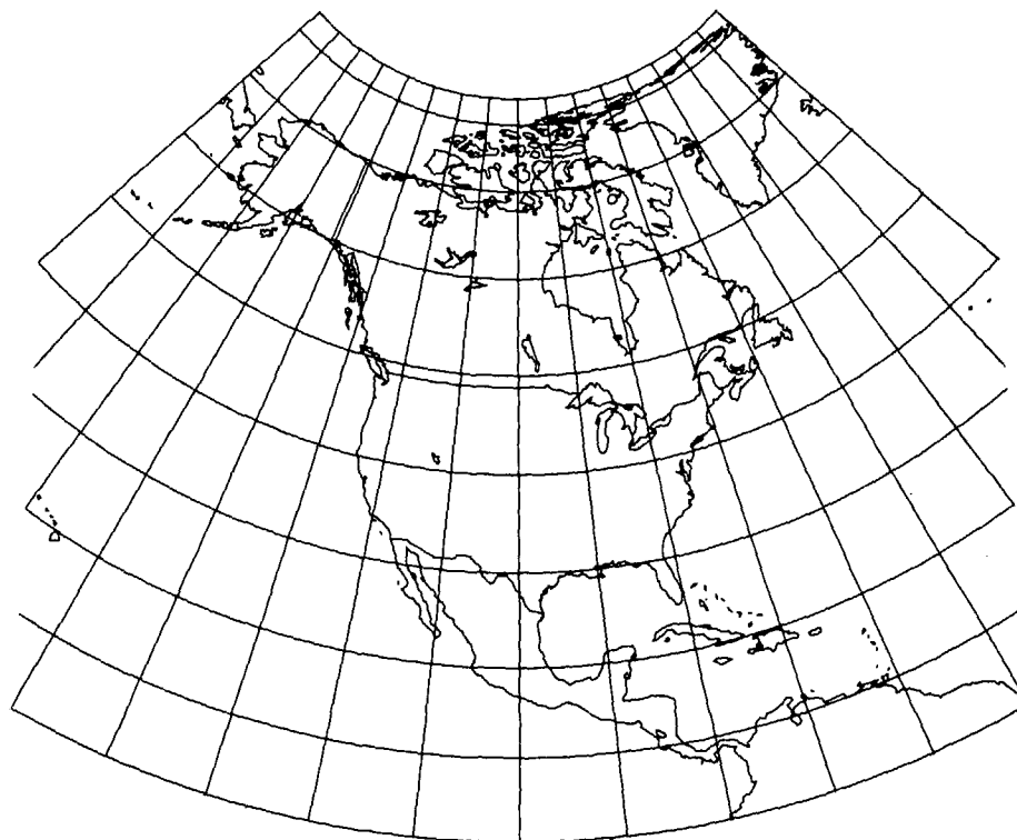
FIGURE 20.—Albers Equal-Area Conic projection, with standard parallels 20° and 60° N. This illustration includes all of North America to show the change in spacing of the parallels. When used for maps of the 48 conterminous States standard parallels are 29.5° and 45.5° N.
