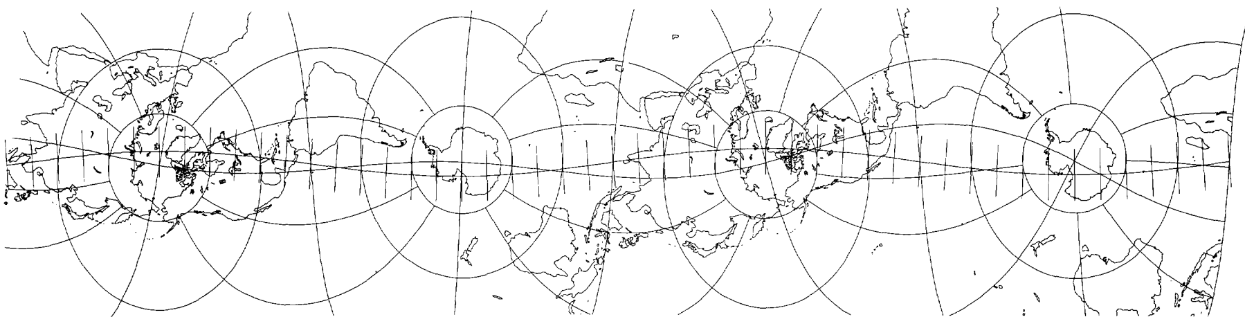
FIGURE 46.—Two orbits of the Space Oblique Mercator projection, shown for Landsat 5, paths 15 (left) and 31. Designed for a narrow band along ground-track, which remains true to scale. Note the rotation of the Earth with successive orbits. Scan lines, extended 15° from groundtrack, are short lines nearly perpendicular to it.
