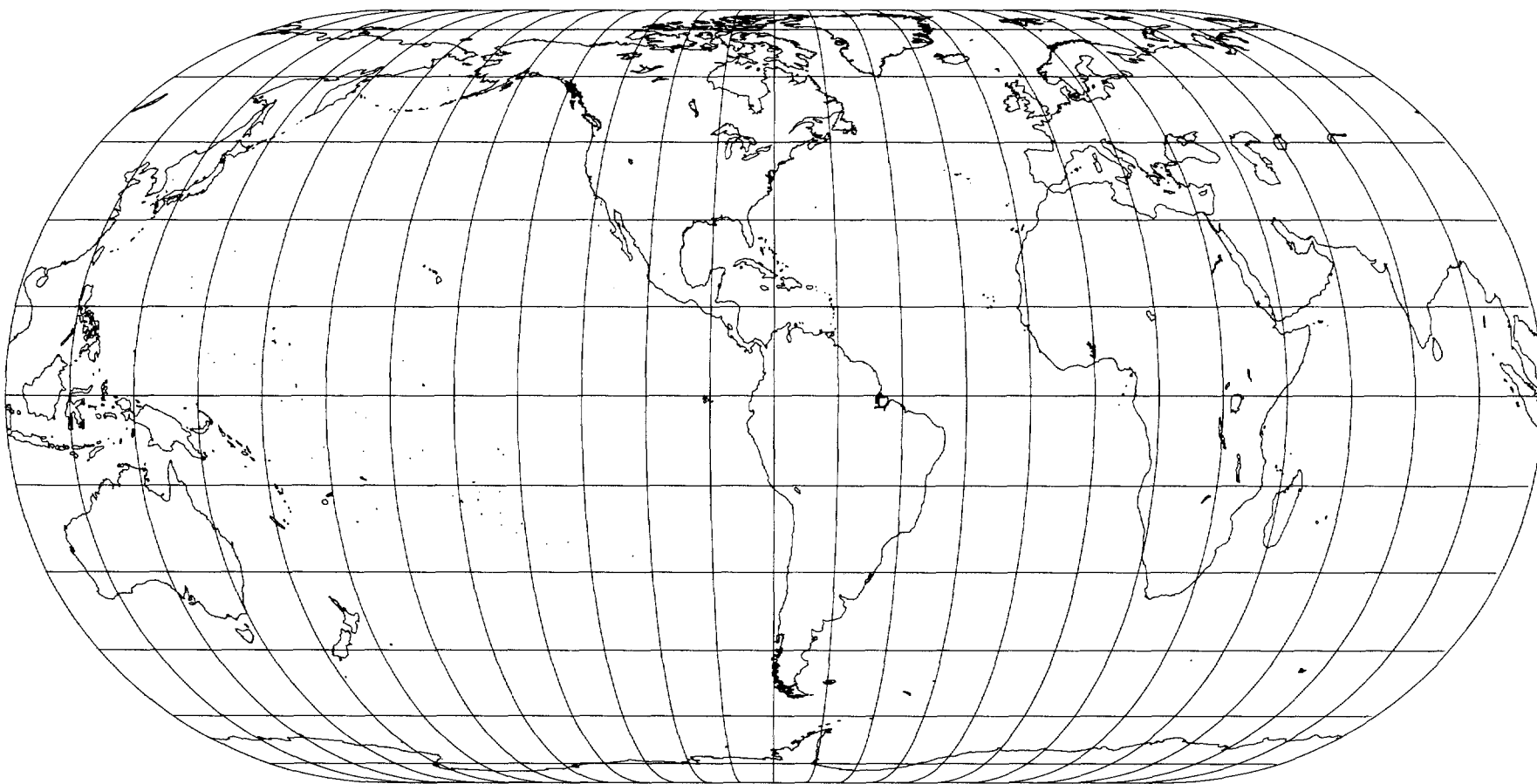
FIGURE 56.—Eckert IV projection. An equal-area pseudocylindrical with poles half the length of the Equator. Outer meridians are semicircles; others are elliptical arcs.
