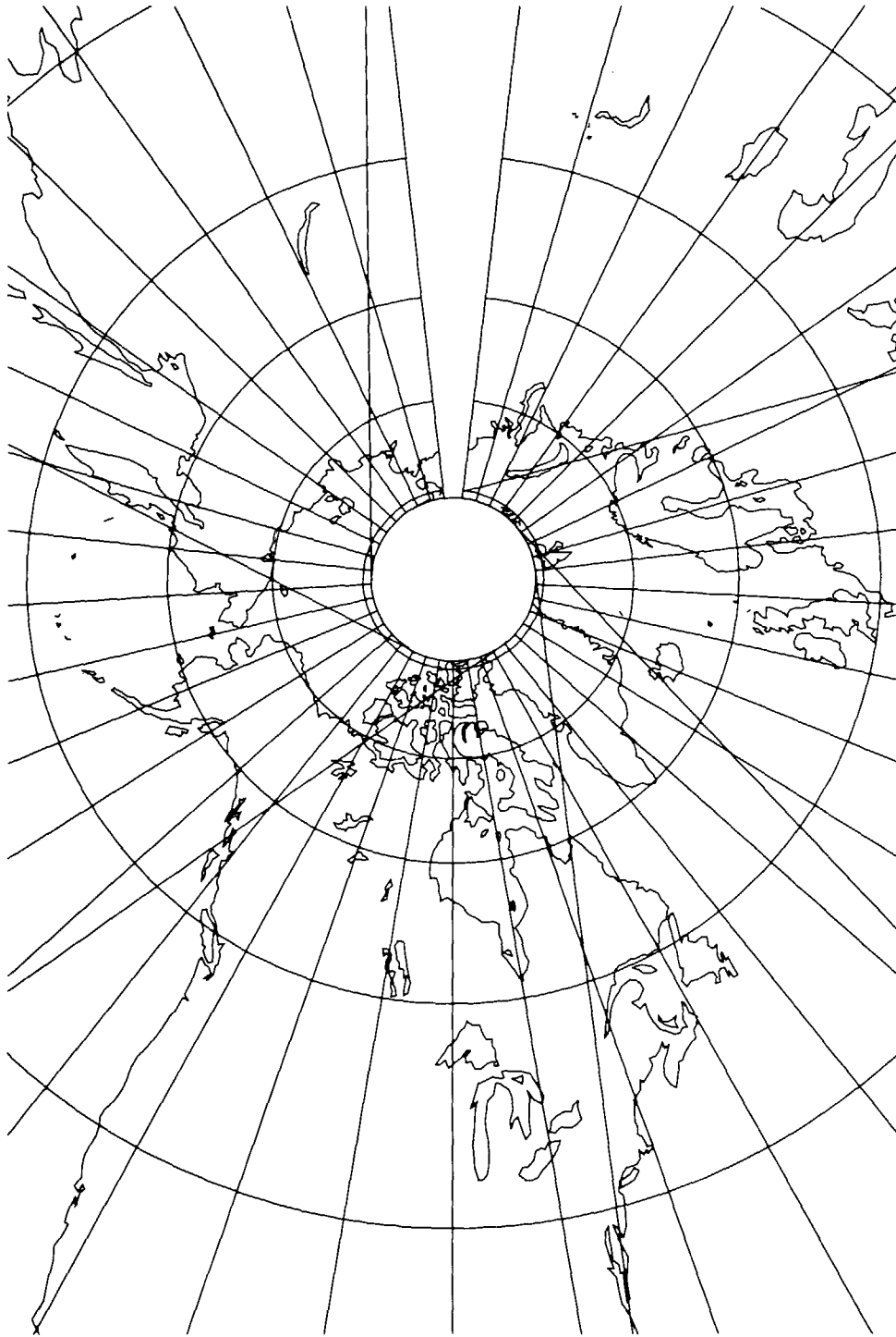
FIGURE 51.—Conic Satellite-Tracking projection (standard parallel 80.9^\circ N.). Landsat 1, 2, 3 orbits. Groundtracks are as described on Fig. 50. The nearest approach to an azimuthal projection for these orbits. Inner circle is tracking limit and circle of tangency.
