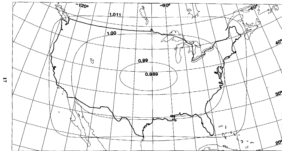
FIGURE 45.—Modified-Stereographic Conformal projection of 48 United States, bounded by a near-rectangle of constant scale. Three lines of constant scale are superimposed. Region bounded by near-rectangle has minimum error.
