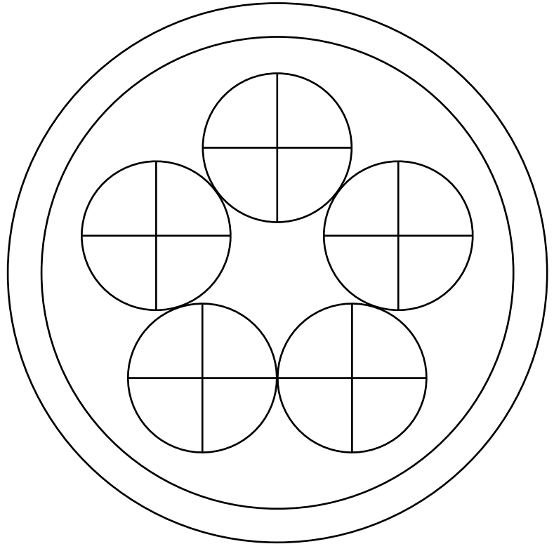
Building to Center Box 3" PVC Cap 3 control line glands 0.9" centers 2 RG-58 bulkheads 0.9" centers
