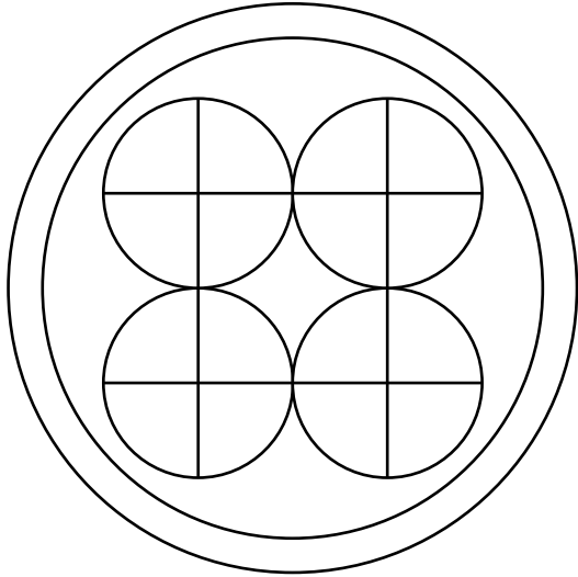
Box to Box 2" PVC Cap 2 control line glands 0.9" centers 2 RG-58 bulkheads 0.9" centers
