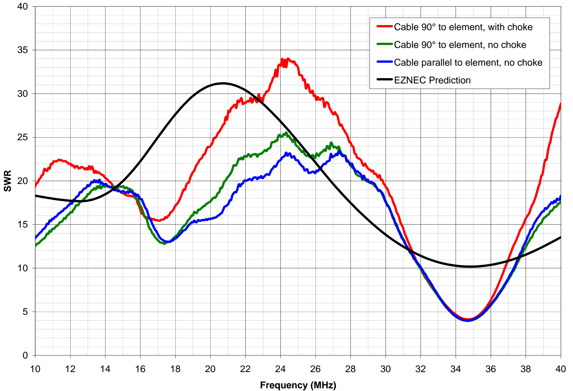
Measured SWR at TFD Feedpoint Terminals – 30' TFD at 9'2" No Ground Plane
