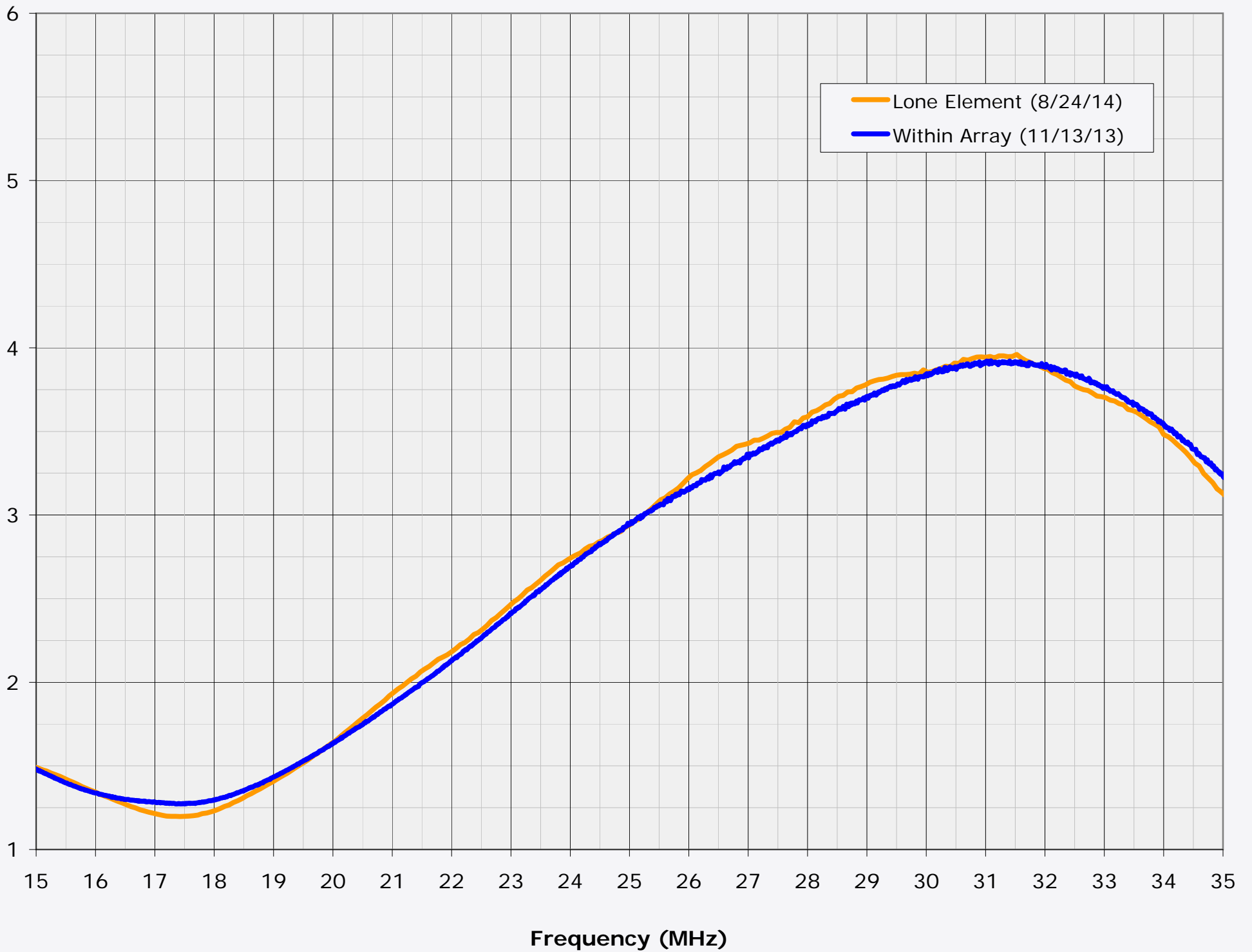
Balun Output SWR
