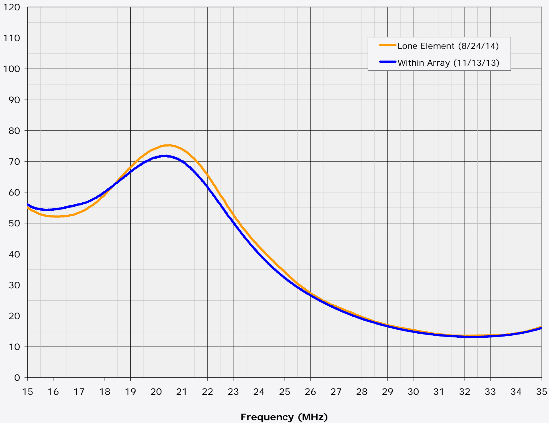
Balun Output R
