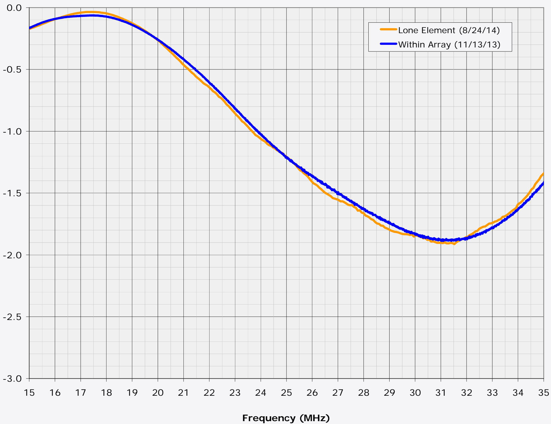
Balun Output Impedance Mismatch Loss
