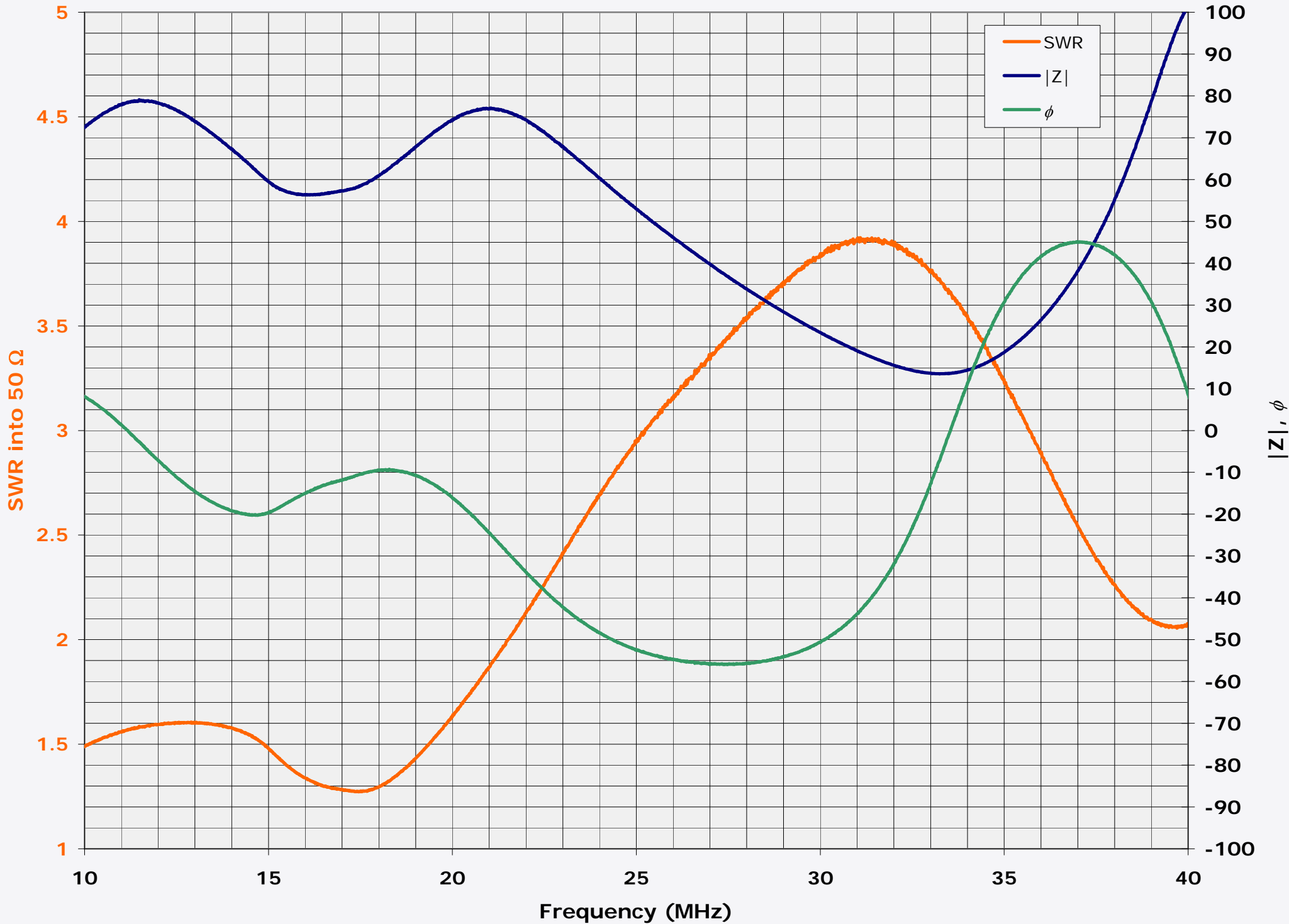
TFD Array Element SWR and |Z| – looking into balun from feed line
