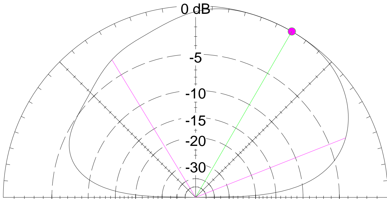
T2FD Antenna
