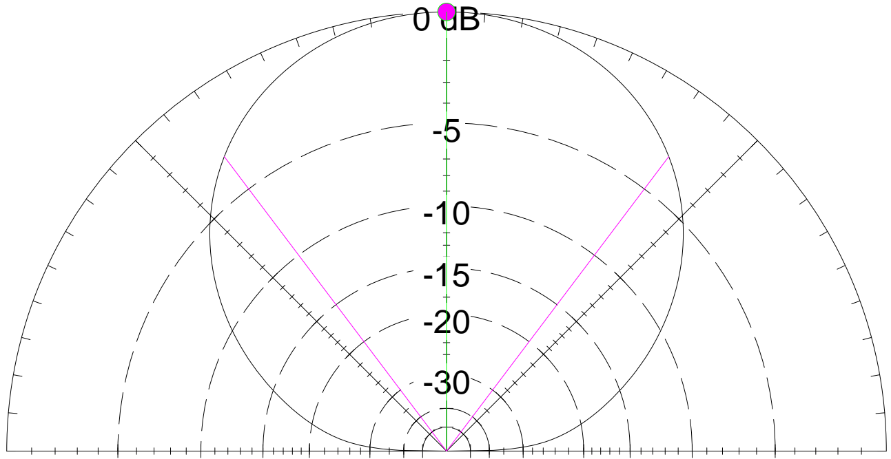
Riometer Zenith Array
