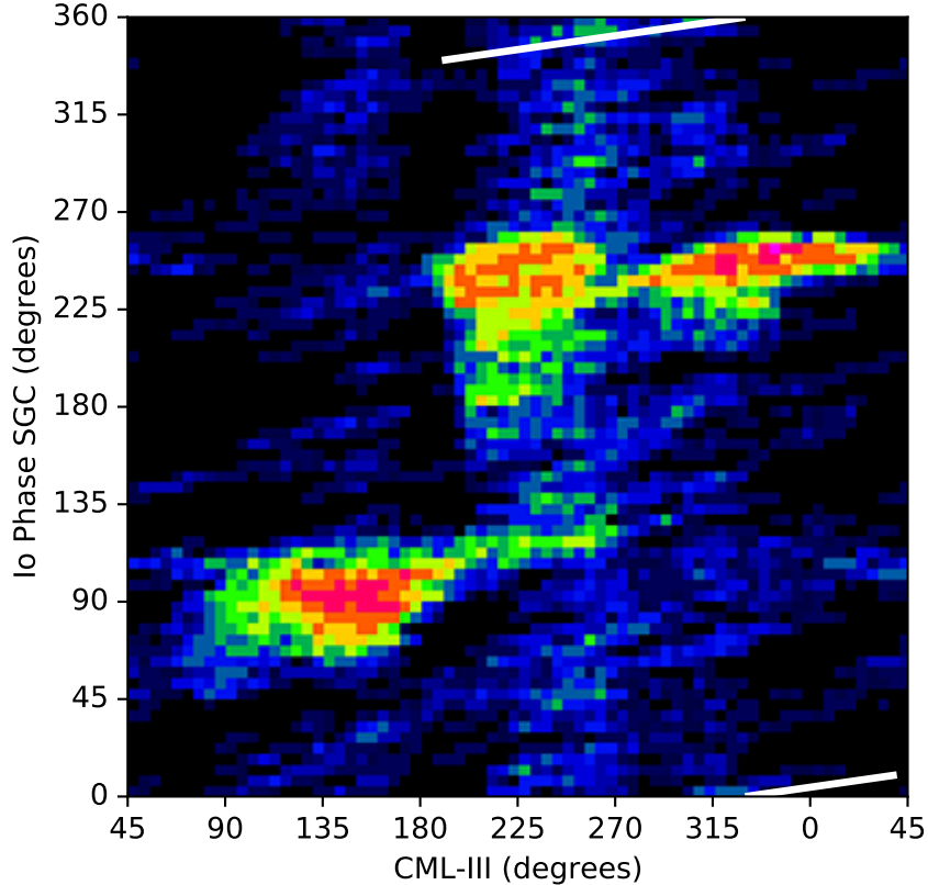
Jovian DAM Track, 24 Jul 2020, 0225 - 0305 UTC
